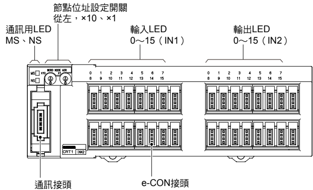
CRT1-ID32S (-1) 型、CRT1-ID32SH (-1) 型
