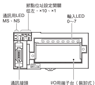
CRT1-ID08TA (-1) 型、CRT1-ID08TAH (-1) 型
