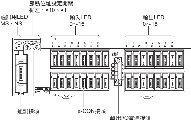
CRT1-MD32S (-1) 型、CRT1-MD32SH (-1) 型
