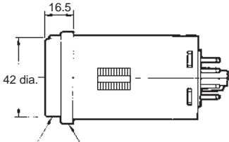
Time setting ring Panel cover
