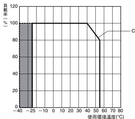
240W/480W/960W <左右間隔不到15mm>
