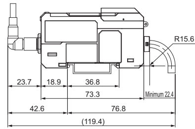
When extension cable (XS3W-M422/M424-□-□) is connected
