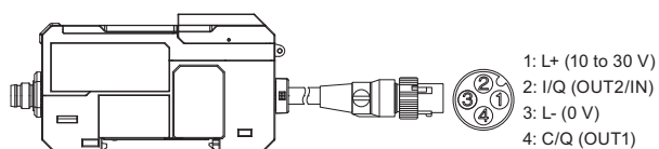
ZP-L3931-IL3 (Pre-wired Connector type)
