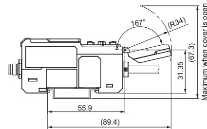
Operating section cover open position (DIN Track mounting)
