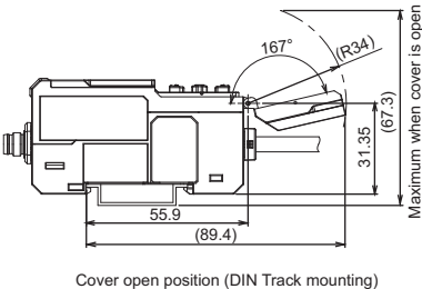
Cover open position (DIN Track mounting)
