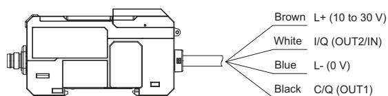
ZP-L3930-IL3 (Cable pull-out type)
