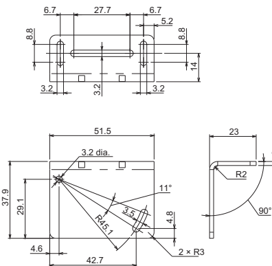
Mounting bracket
