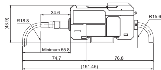
When extension cable (XS3W-M421/M423-□-PR) is connected
