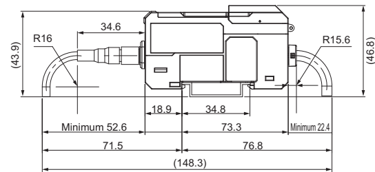
When ZP-LS□ and extension cable (XS3W-M421/M423-□-R) are connected
