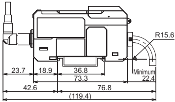
When extension cable (XS3W-M422/M424-□-□) is connected
