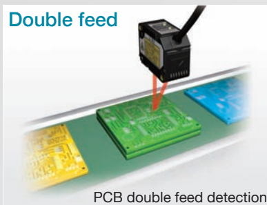
PCB double feed detection
