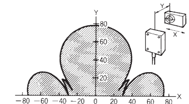
V600-HS63 + V600-D8KR04
