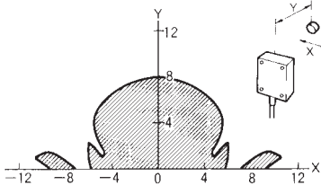
V600-HS61 + V600-D8KR12D
