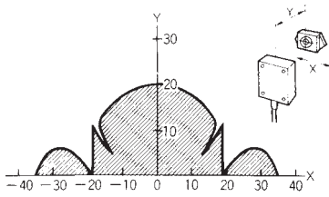
V600-HS63 + V600-D23P71
