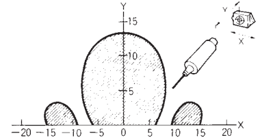
V600-HS51 + V600-D23P61
