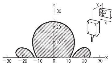
V600-HS61 + V600-D8KR12D
