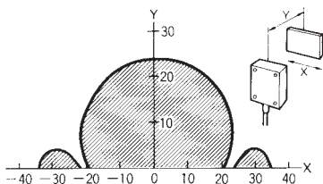
V600-HS61 + V600-D23P72
