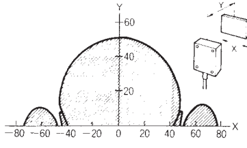
V600-HS63 + V600-D8KR13
