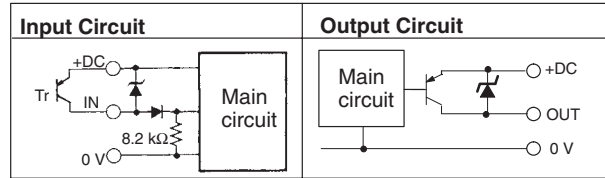
V600-HAM81
