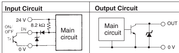
V600-HAM91
