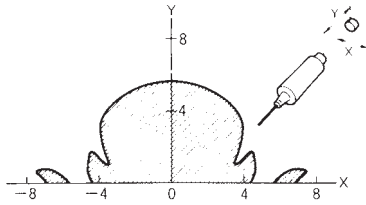
V600-HS51 + V600-D8KR12D
