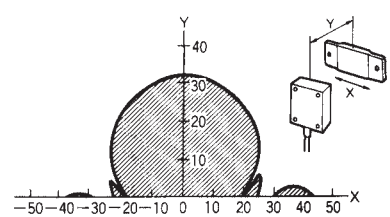
V600-HS63 + V600-D8KR12D
