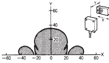
V600-HS63 + V600-D8KR13
