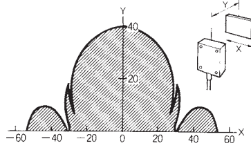
V600-HS63 + V600-D2KR16
