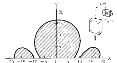
V600-HS61 + V600-D23P61
