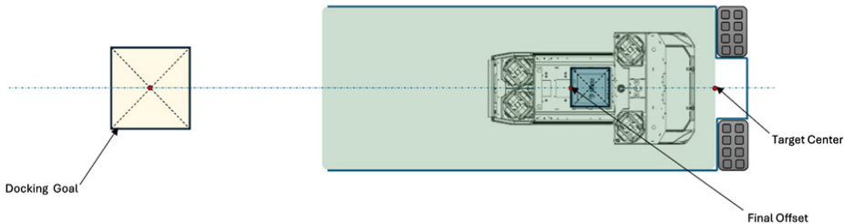
Figure 5 -11 Final Approach, OL-450S2
