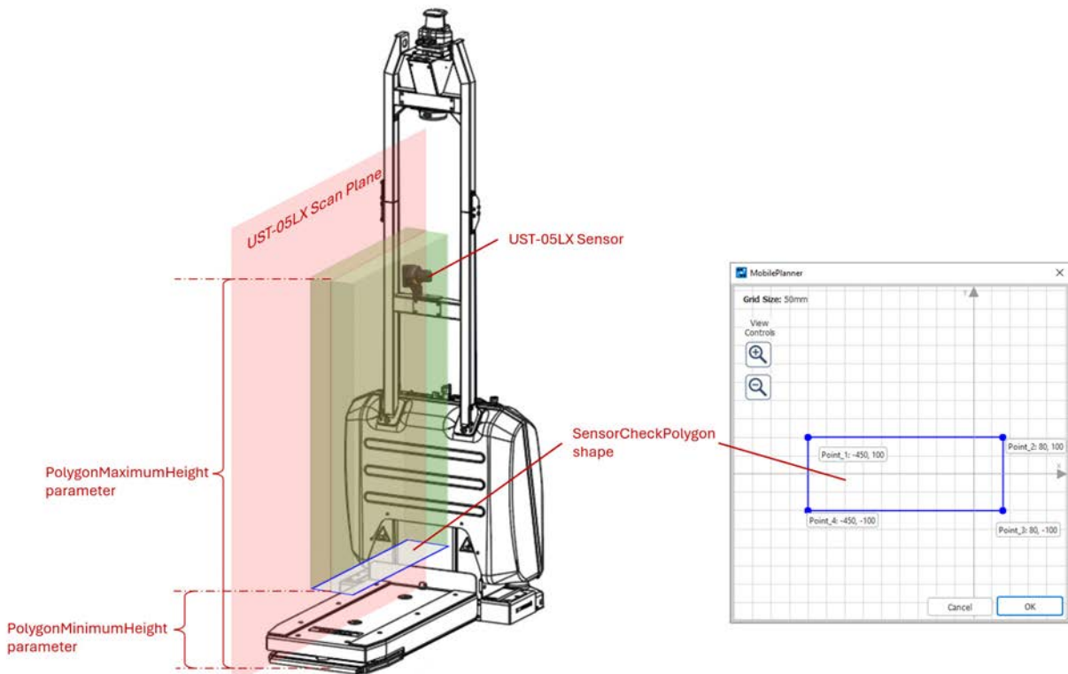
Figure 7-3 In-Transit Monitoring Scanner Region
