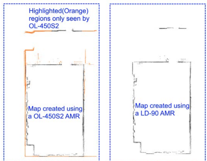
Figure 3-6 Maps Generated by an OL-450S2 and a LD-90
