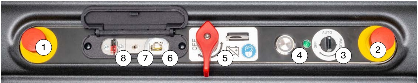
Figure 2-1 OL-450S Control Strip
