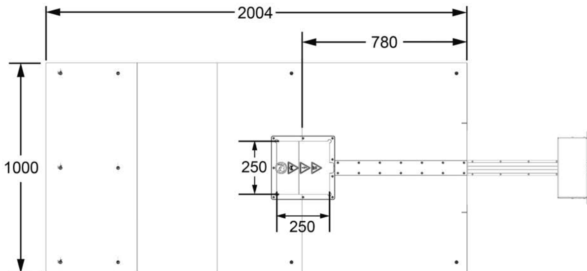
Figure 5-5 Charger Ramp Dimensions
