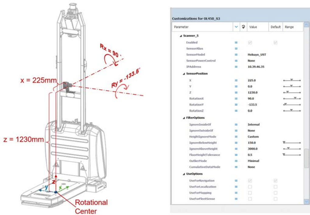
Figure 7-2 Configuring Scanner Settings
