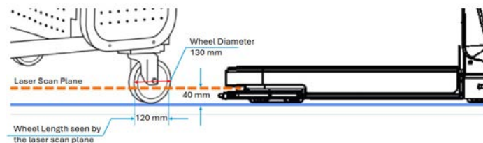
Figure 6-5 Wheel Length Scanned by the Rear Scanner
