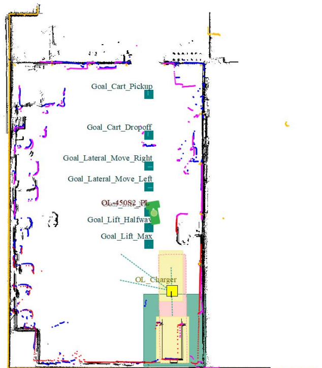
Figure 3-5 “OL-450S.map” Created Map File
