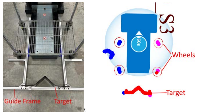
Figure 6-14 Target on a Guide Frame
