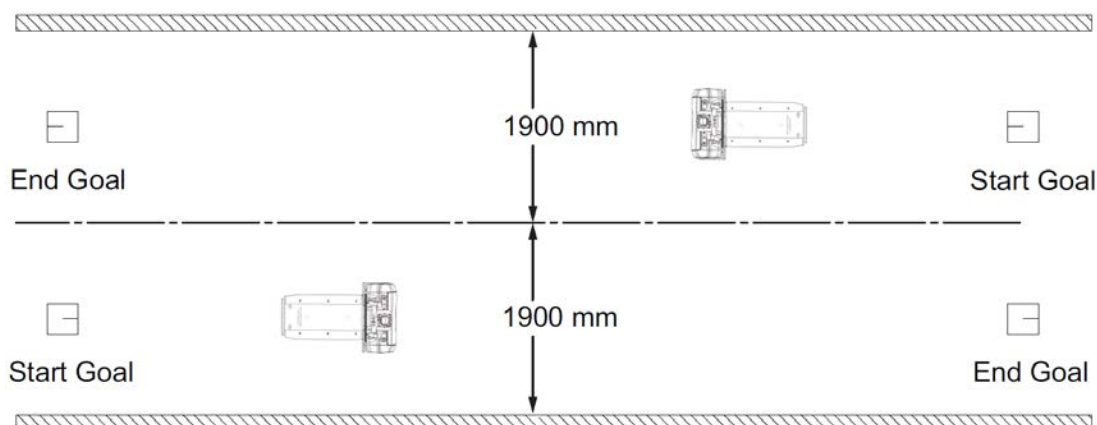
Figure 4-2 Minimum Lane Requirement to Maintain Maximum Speed
