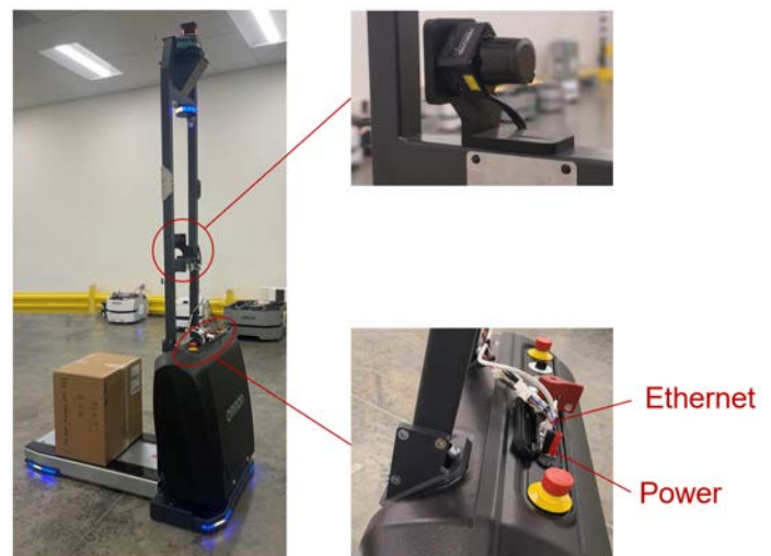
Figure 7-1 HOKYUO UST-05LX Scanner Placement and Connections
