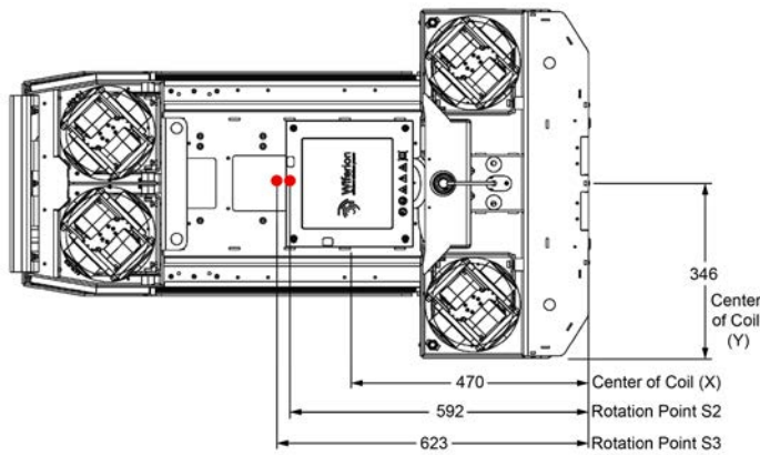
Figure 5-6 OL-450S Rotation Point and Center Of Charging Coil
