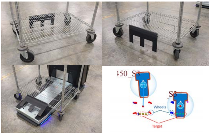
Figure 6-13 Cart with Flexible Target
