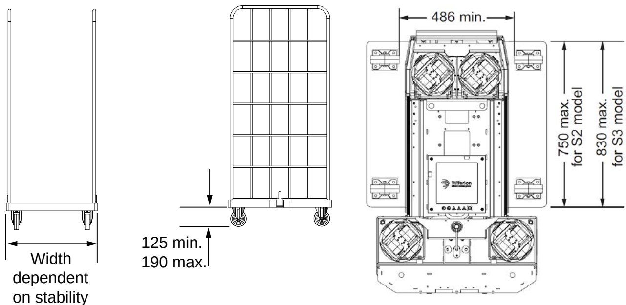
Figure 6-1 Load Carrier Specification Requirements
