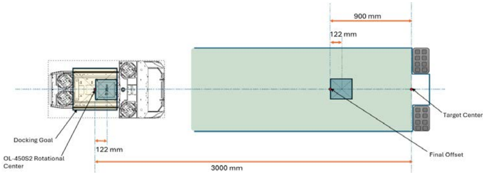
Figure 5-10 Custom Target Layout, OL-450S2
