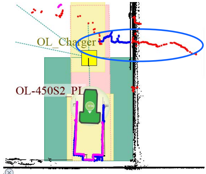
Figure 5-16 Rear Scanner Detecting Floor As Obstacle
