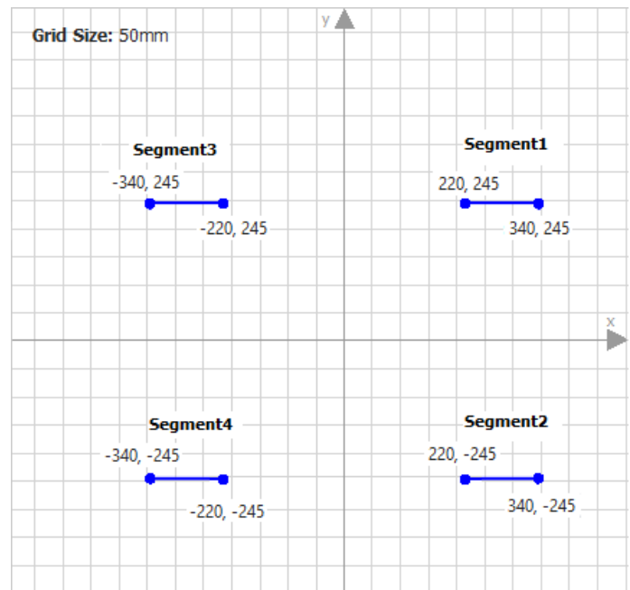
Figure 6-6 Four Line Segments to Represent Cart Target Definition
